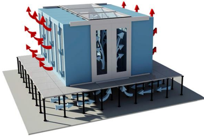
Cold-Aisle Containment
