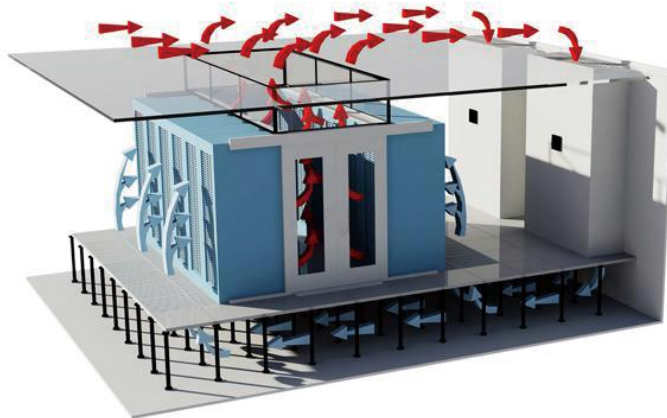
Hot-Aisle Containment
